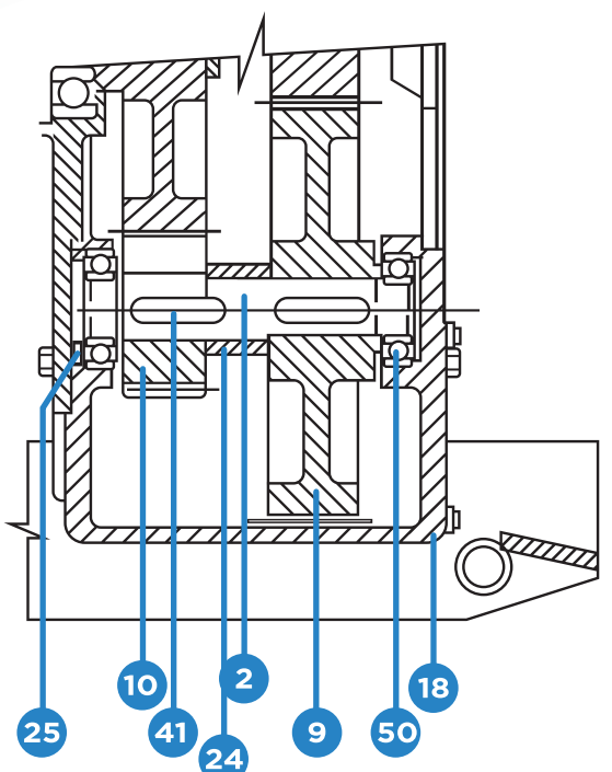
ALTERNATIVE LAY SHAFT ASSEMBLY
